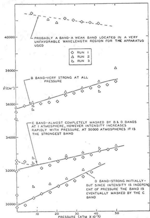
Fig. 2(a). The effect of pressure on the spectra of color centers in NaCl: 1.0% AgCl, Part 1.
